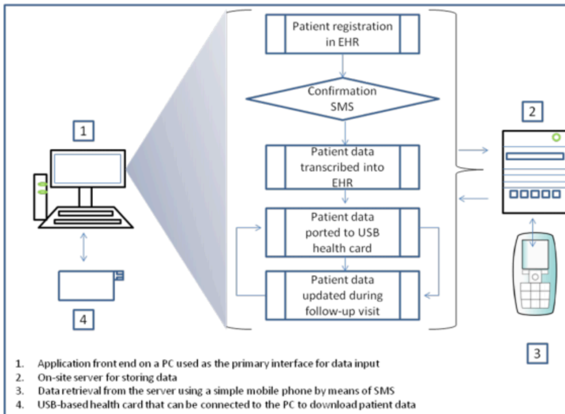
Figure 2: System Workflow
